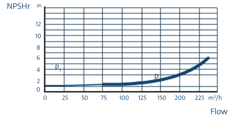
The NPSH curve requirement from the pump manufacturer
